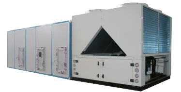
Direct expansion air conditioning unit Environmental refrigerant: R410A/R407C Rated cooling capacity : 14.5-720kW
